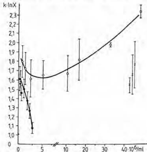
Fig. 12 — The decay parameter of the hyperbolic approximation that is adjusted to the relaxation dynamics of the afterglow of different cell suspensions after exposure to weak white light illumination is shown versus cell density. The lower curve displays the improvement of hyperbolic relaxation of normal amnion cells with increasing cell density. The upper curve shows the opposite dependence exhibited by malignant Wish cells. The three measurements at the right side of the figure correspond to the nutritive medium alone.
