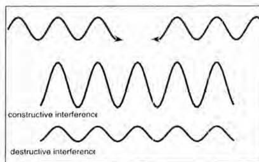
Fig. 9—If two waves interfere, the phase relations will lead in general to zones where they amplify mutually ("constructive interference") or alternate ("destructive interference"). For coherent fields, these processes provide a basis of regulation and communication.
