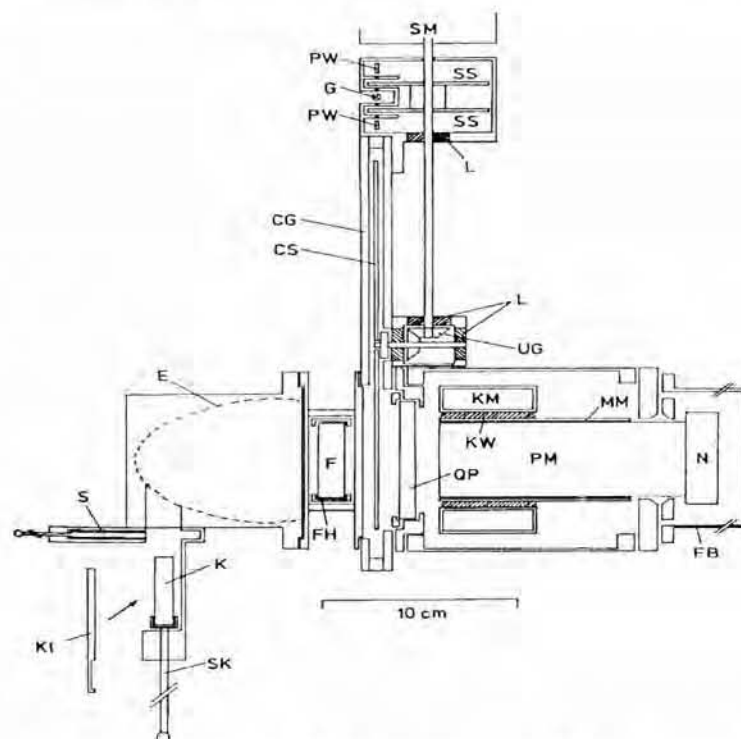
Fig. 3— The measuring equipment. PM—photomultiplier; CS—disc of the chopper; CG—housing of the chopper-disc; E—ellipsoid; F—filters; FB—faraday cup; FH—filter holder; G—lamp; K—test quartz glass; KI—flap; L—ball bearing; KM—cooling jacket; KW—Copper wool; MM—metal cylinder; N—network; PW—photosensitive resistor; QP—quartz glass; S—slide to close the ellipsoid; SK—rod to move up the test glass; SM, UG—geared motor; SS—sector-discs.
