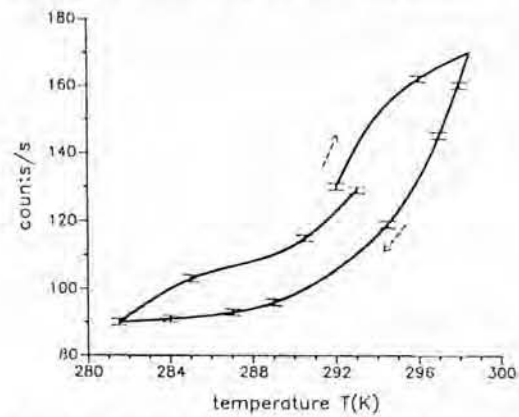
Fig. 7— The biophoton intensity of living tissues shows a hysteresis-like dependence on the temperature T , if T is cyclically varied. The example shows etiolated barley, 4 days of germination. The variation of temperature starts at T=292 K with the rate \partial T/\partial t=0.5 K/min. At T=298.5 K the rate of temperature change is reversed to \partial T/\partial t=-0.5 K/min, and again at T=281.5 K with \partial T/\partial t=0.5 K/min. This hysteresis-like behaviour of biophoton intensity can truthfully be described as a Curie-Weiss-law-dependence.
