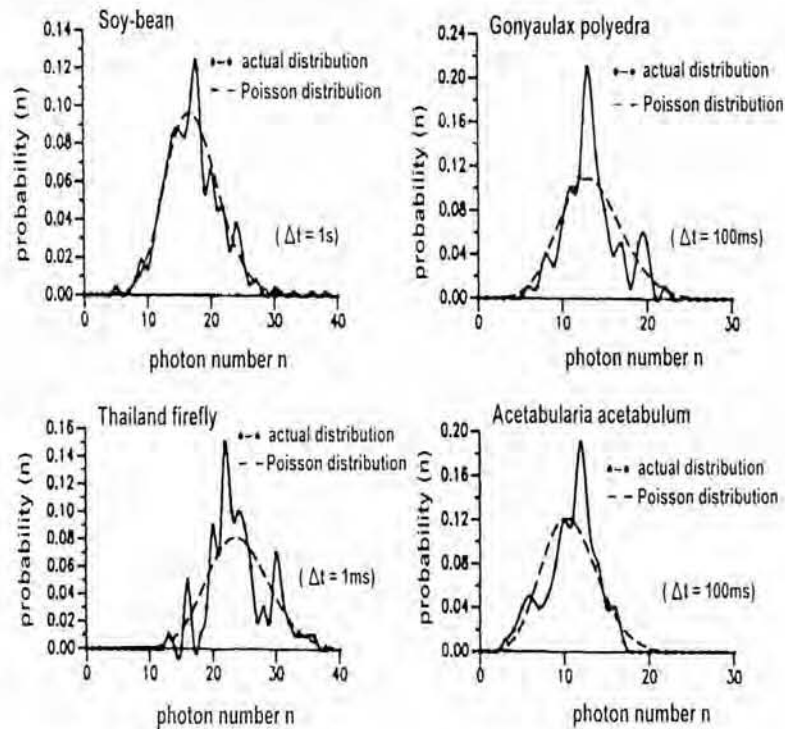
Fig. 5— The photocount statistics (=probability p(n, \Delta t) of registering n counts in a preset time interval \Delta t , where n=0, 1, 2, \dots ) is very similar for all biological systems. If \Delta t is sufficiently small such that the mean number of photons in the field becomes lower than about 100, p(n, \Delta t) displays a Poissonian (and sometimes even a sub-Poissonian) photocount distribution. There are 4 different examples with different \Delta t . 100 measurement values have been used always for evaluation, where the biological state was kept quasi-stationar.
