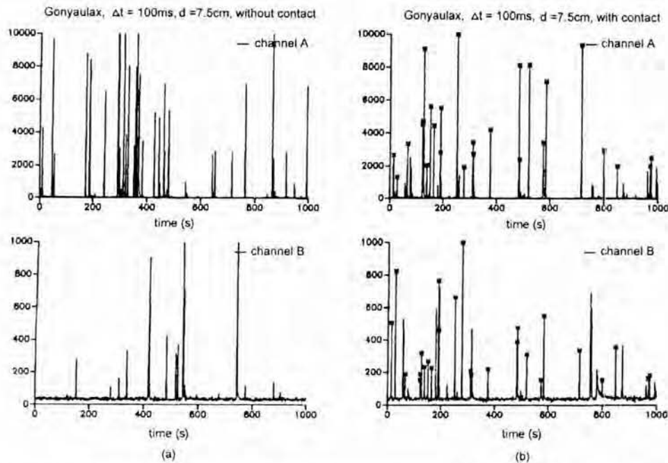
Fig. 13 — If ones separates two cultures of dinoflagellates, their bioluminescence flickering is completely unsynchronous (left side). As soon as they are in optical contact, a big amount of flickering is synchronous (right side). The stars indicate the synchronous flashes.
