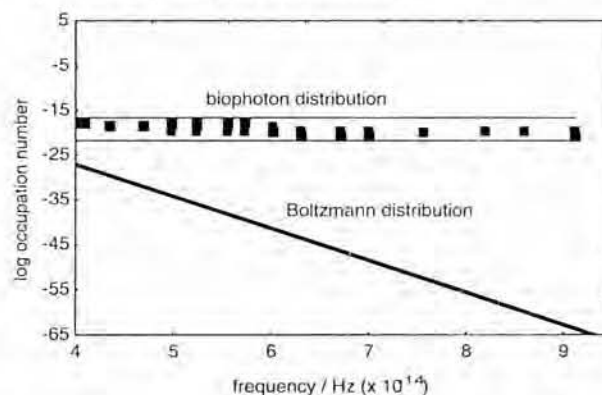
Fig. 4— In the case of average occupation numbers we obtain a l = \text{const.} -distribution that with increasing frequency displays increasing deviation from the Boltzmann-distribution.
