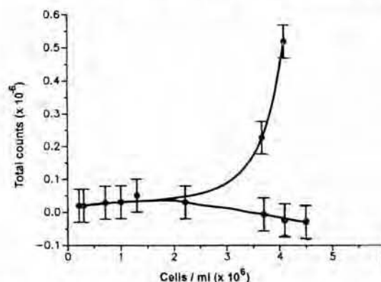
Fig. 11—"Delayed luminescence" from tumor cells (upper curve) and normal cells (lower curve), as measured by Schamhart. The different curves can be approximated by a non-linear (cubic) dependence of intensity from cell-number n .
