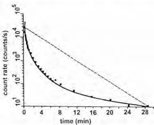
Fig. 6— Instead of an exponential decay (dashed line), living cell populations (here tissue of Bryophyllum daigremontanum ) exhibit a hyperbolic relaxation of photon intensity after exposure to white-light-illumination. This holds for total as well as for spectral observation (here at 676 \pm 10 nm). Under ergodic conditions, hyperbolic decay is a sufficient condition of perfect coherence.
